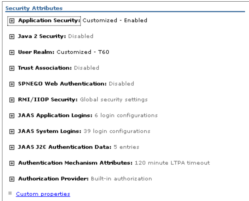
Figure 3-6 Security attributes section of the security domain configuration page
