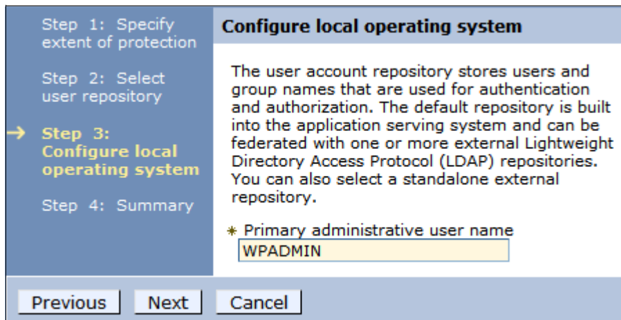
Figure 11-3 Step 3: Configure local operating system
