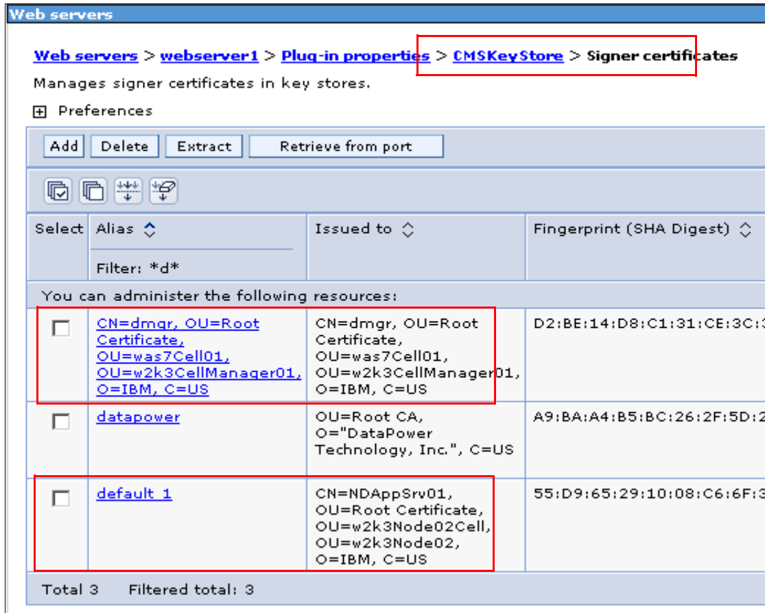
Figure 5-29 Filtered list of signer certificates
