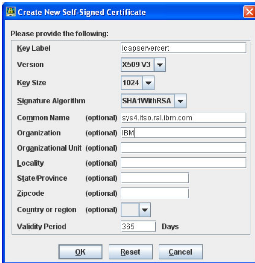
Figure 5-19 Create self-signed certificate
