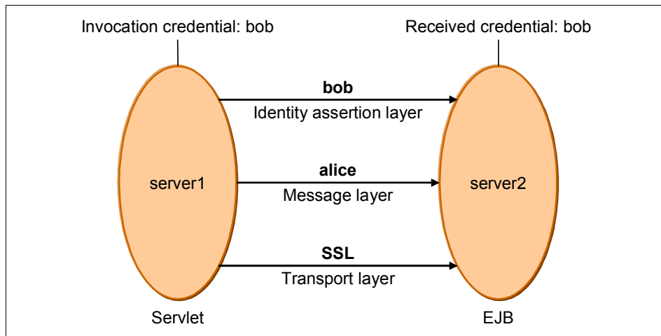
Figure 6-4 Case study 1: Servlet calling an EJB using identity assertion
