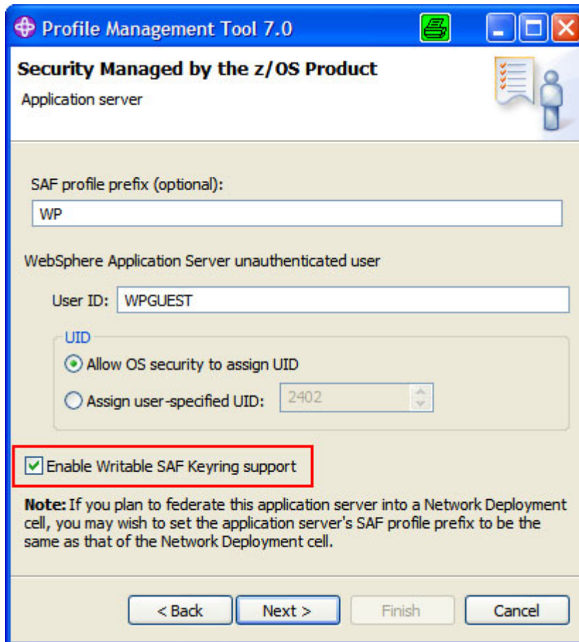
Figure 13-6 Enable Writable SAF Keyring support during customization
