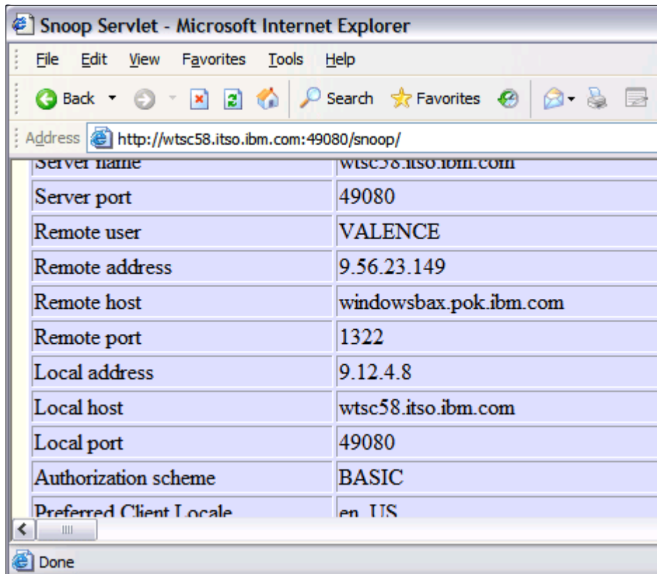
Figure 12-6 Snoop servlet showing authenticated RACF user ID
