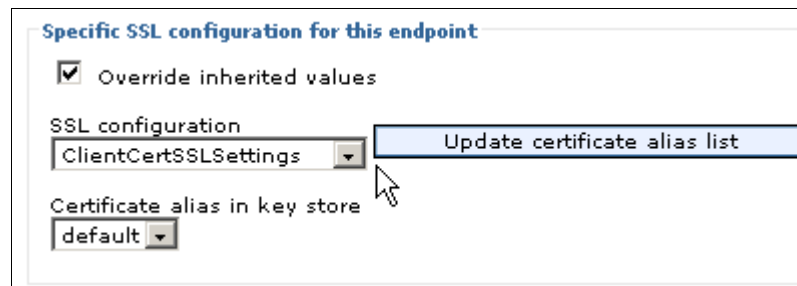
Figure 8-23 Selecting the SSL configuration
