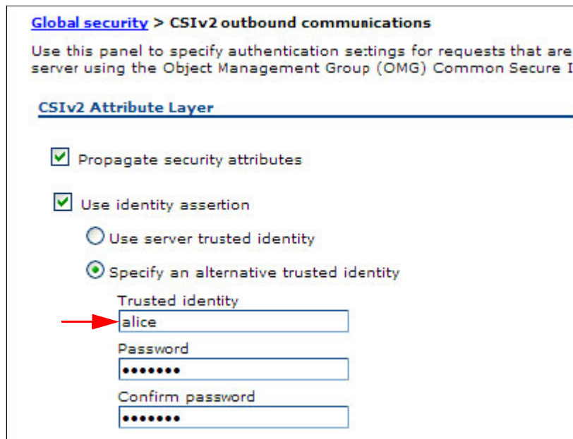
Figure 6-5 Case study 1: CSIV2 outbound settings on the sending server
