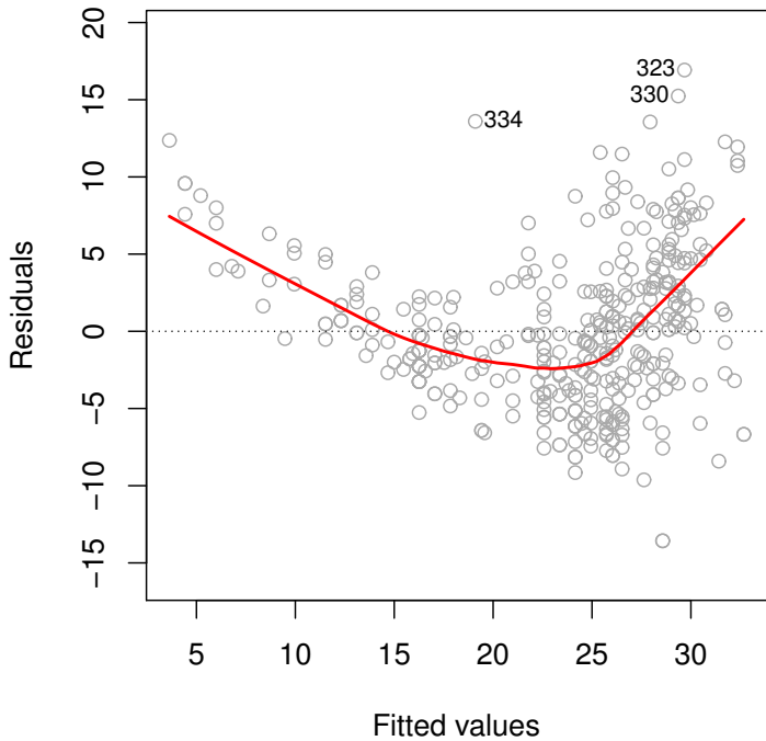
Residual Plot for Linear Fit
