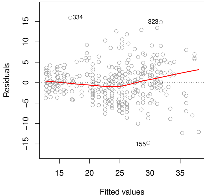
Residual Plot for Quadratic Fit
