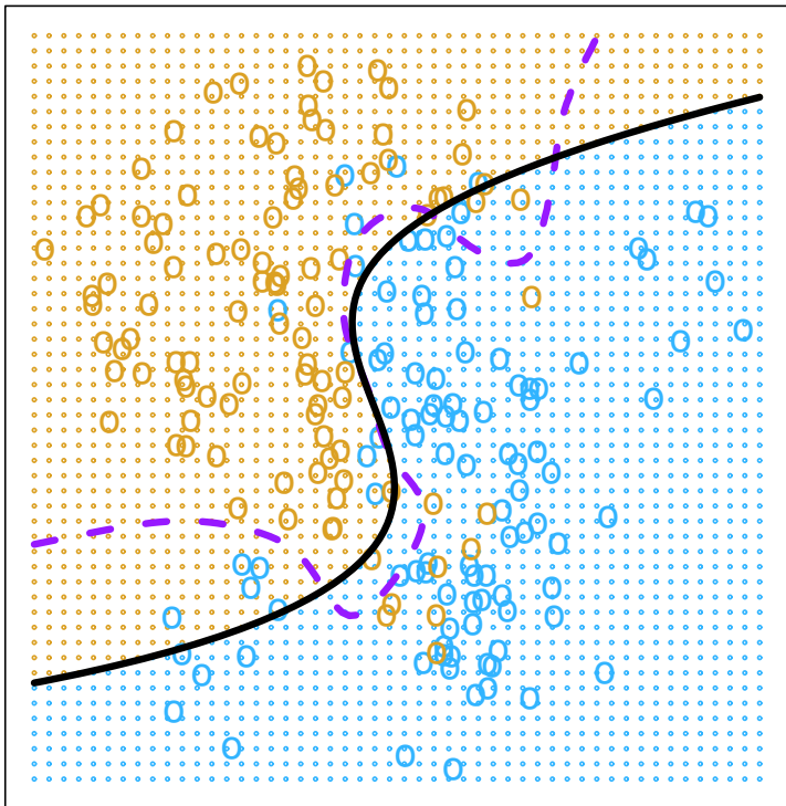
Degree=3
