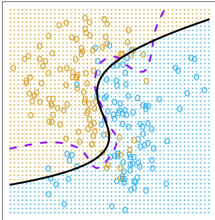
Degree=4
