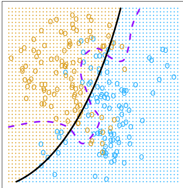
Degree=2
