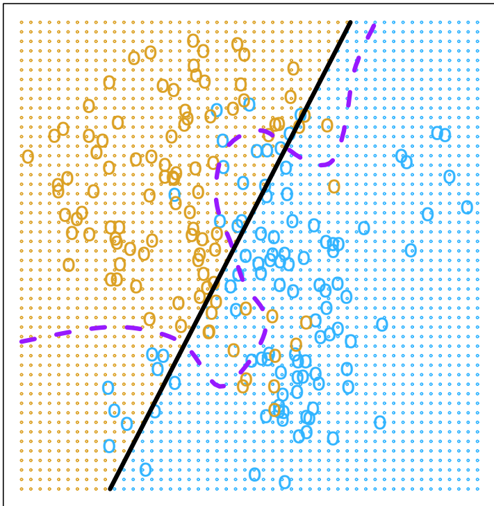
Degree=1
