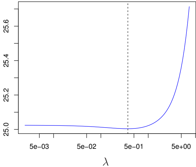
Cross-Validation Error
