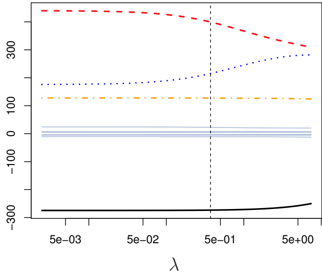
Standardized Coefficients
