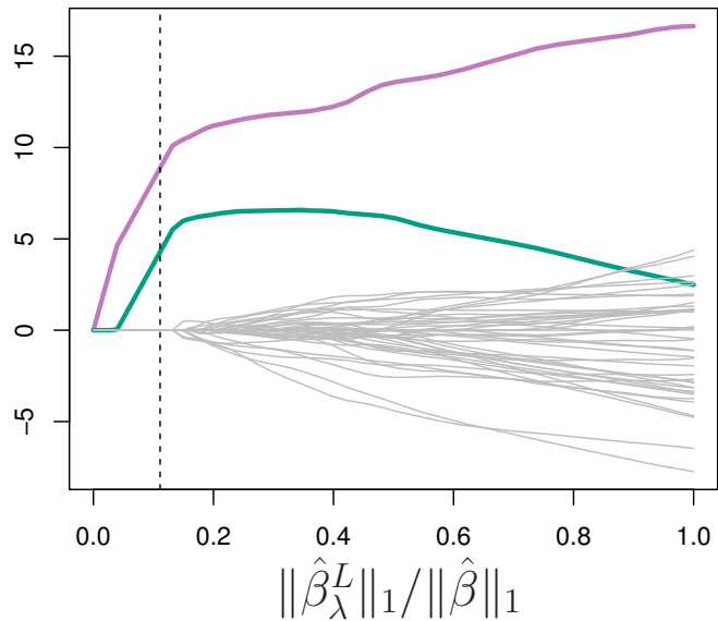
Standardized Coefficients
