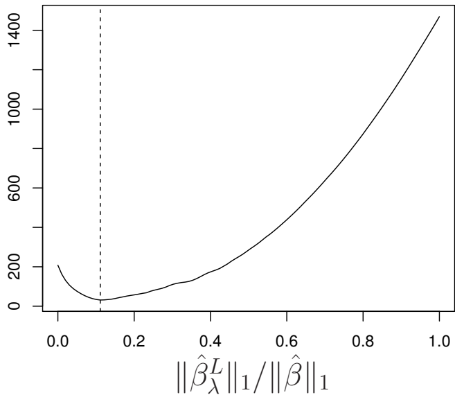
Cross-Validation Error
