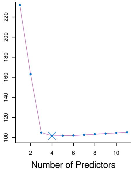
Square Root of BIC
