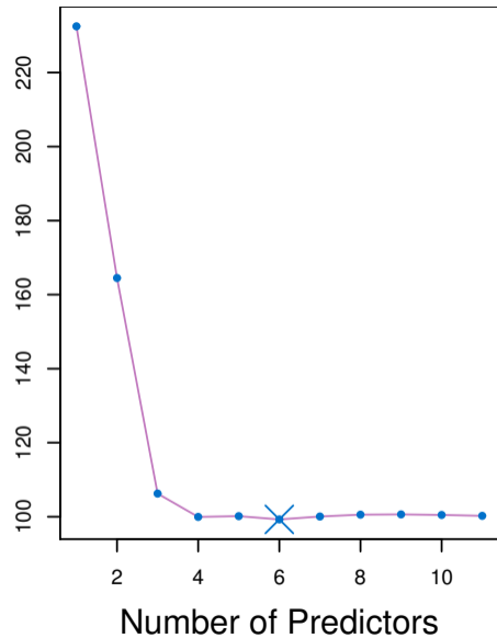
Cross-Validation Error
