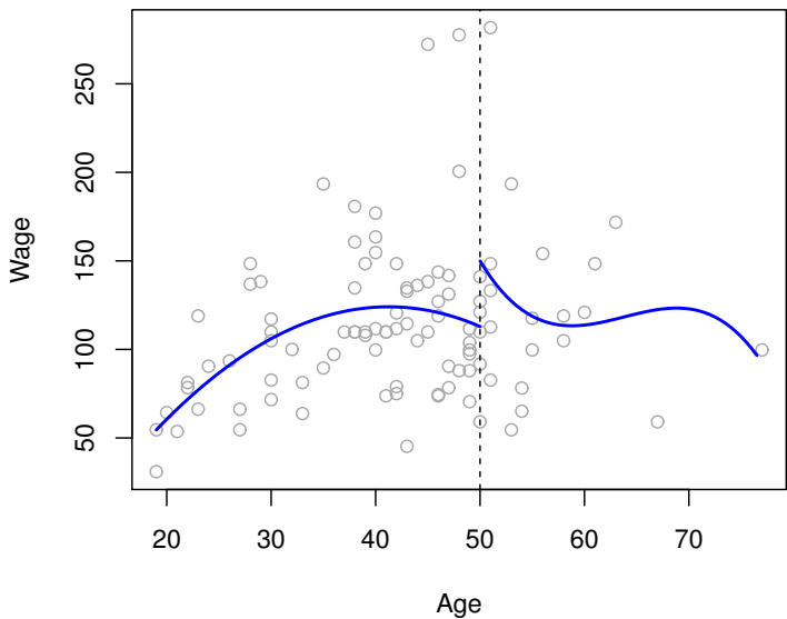
Piecewise Cubic
