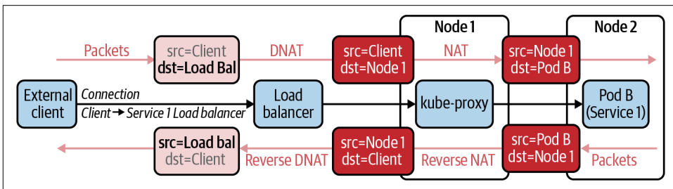
Figure 9-3. Network path for a Kubernetes service of type LoadBalancer
